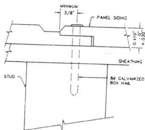
DRAWING 6C GROOVED PANEL SIDING WIDE SHIP LAP JOINT Fastening when racking resistance is provided by siding
