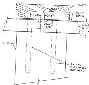
DRAWING 6B GROOVED PANEL SIDING WIDE SHIP LAP JOINT Normal fastening where racking resistance is provided by sheathing or bracing
