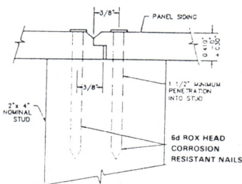
DRAWING 6D STUCCO/CYPRETEX PANELS SHORT SHIPLAP JOINT DETAIL Fastening when racking resistance is provided by siding
